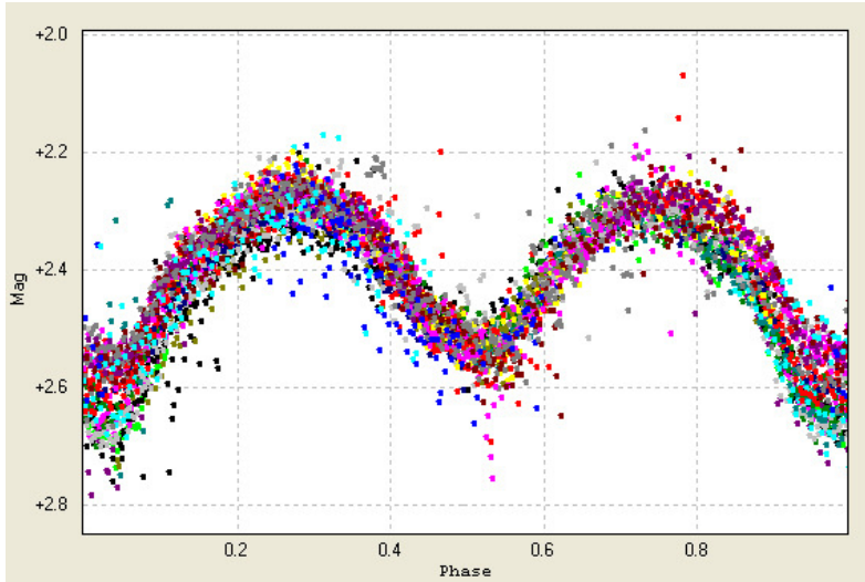
Fig. 2. Phase diagram for the star HMB11 = USNO-B1.0 1249-0502361. The different colours are the different observing runs.
