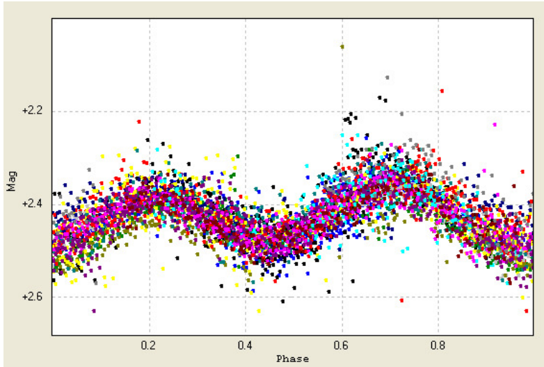
Fig. 3. Phase diagram of HMB12 = USNO-B1.0 1250-0498893. The different colors are for the different observing nights.
