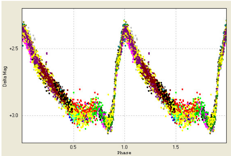
Fig. 4. Phase diagram of HMB13 = USNO-B1.0 1251-0501729. The different colors are for the different observing nights.
