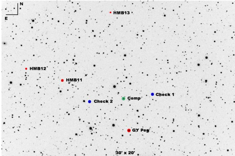
Fig. 1. Finding chart of the new variables (red circles) including comparison (green circle) and check stars (blue circles). The star is indicated by the red circle. GY Peg is also given.
